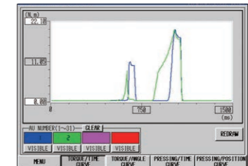
Torque Curve Monitor
